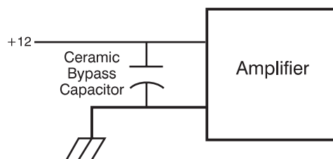
Figure 6.6. RF bypassing the power supply lines.
