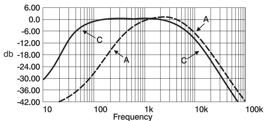
Figure 3.3. A and C weighting filter response curves
